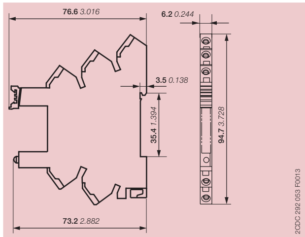
Base rasante CR-S
